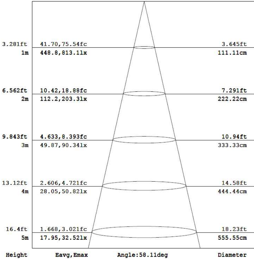
LUMINOUS INTENSITY DISTRIBUTION DIAGRAM
